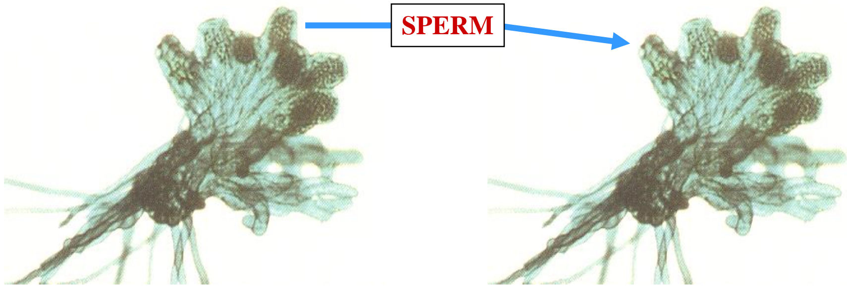
2 ND GAMETOPHYTE
