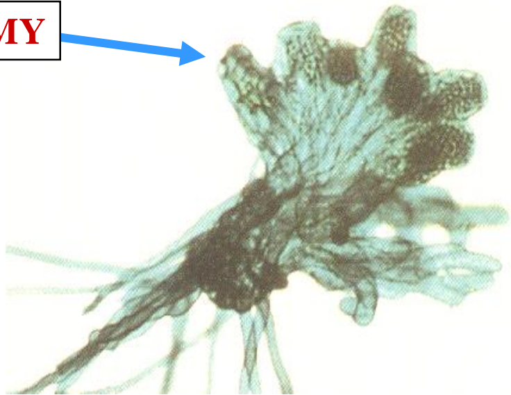
1 ST GAMETOPHYTE
