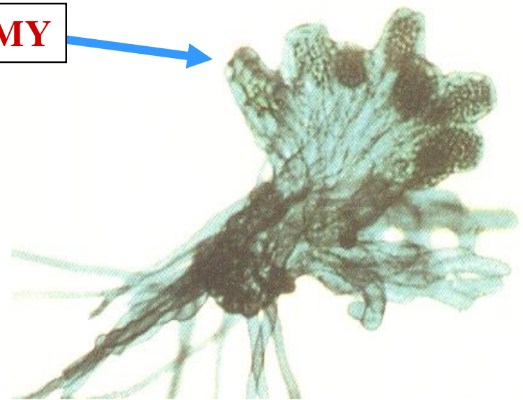
1 ST GAMETOPHYTE
