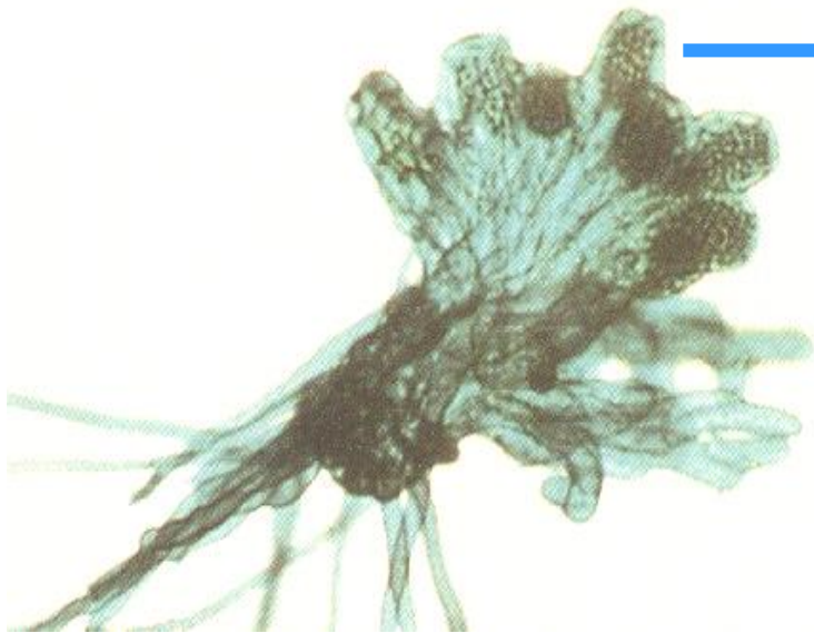
2 ND GAMETOPHYTE
